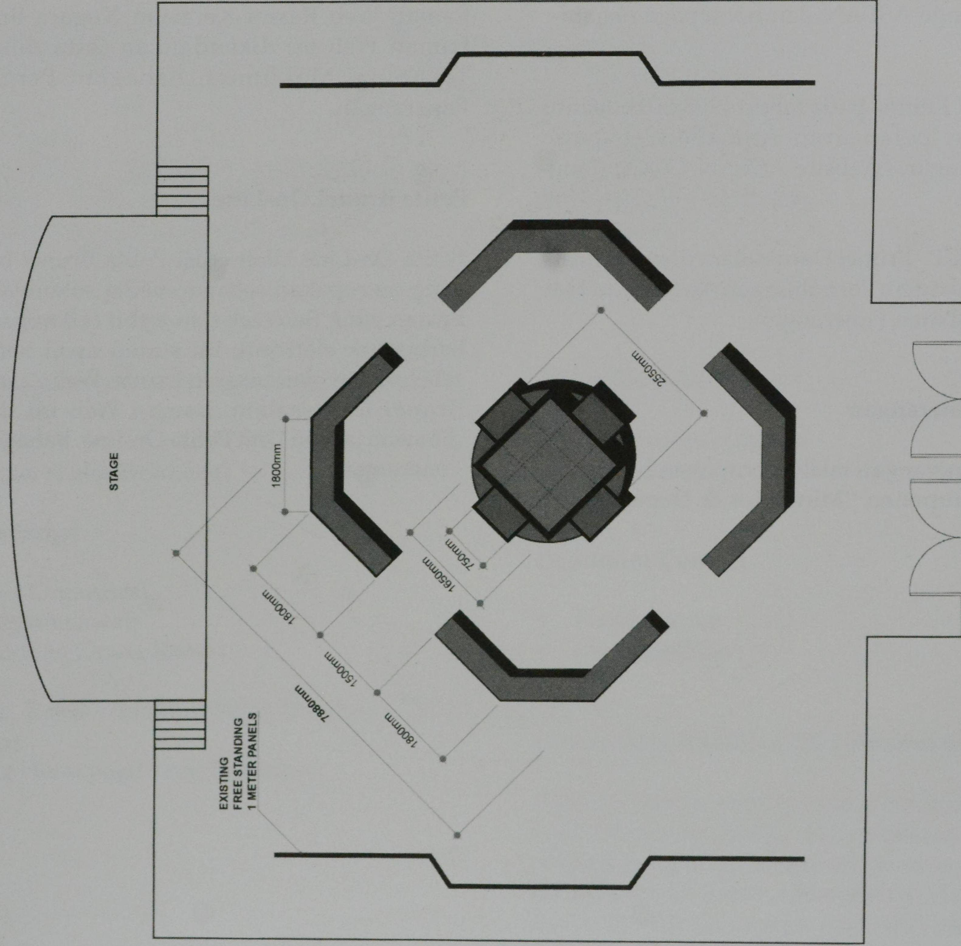
PROPOSED PLAN FOR EXHIBITION BOOTH SCALE: N.T.S.
